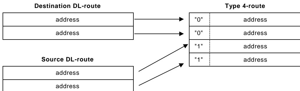
Figure 17 – Extended Type 4-route generation
